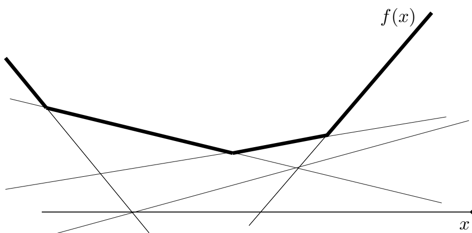
Figure 3: A piece-wise linear convex function
