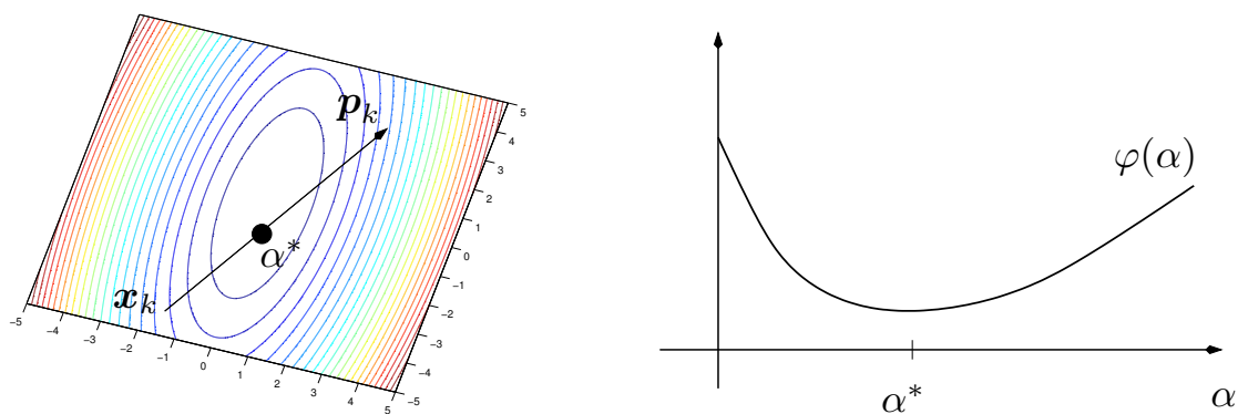
Figure 1: A line search in a descent direction
