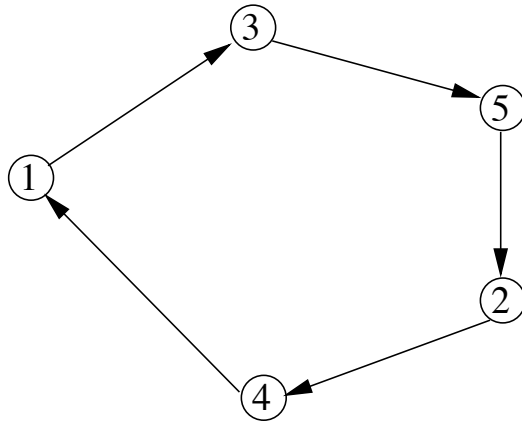
Figure 3: (Exercise 9) An example of a TSP tour with 5 cities. Here x_{13} = 1 , x_{35} = 1 , x_{52} = 1 , x_{24} = 1 and x_{41} = 1 all other variables x_{ij} = 0 .
