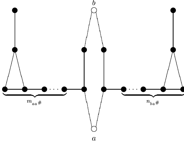
Figure 2: The graph \Gamma_{a,b} .
