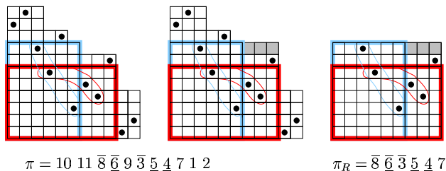
FIGURE 6. Left: A placement p , its \mathcal{A} - and \mathcal{B} -sequences (for k = 3 ), and the rectangles R_A and R_B . Center: The placement p^R . Right: The placement p_R and the corresponding subsequence of \pi .
