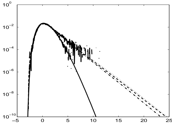
Fig. 5. Example 3: The dashed lines (3 in number) indicate the crossing intensities \mu_N^s(u) using the proposed hybrid method, with sample size for simulated gamma processes \gamma_i is N = 1000 ; the corresponding irregular solid line is MC estimate; The thicker solid line is the saddle point estimate \mu^s(u) with Gaussian forcing; the corresponding irregular solid line is the corresponding MC estimate.
