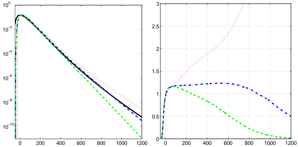
Fig. 4. Example 2: (a) Crossing intensities \mu_N^s(u) computed using the proposed hybrid method: Sample size for simulated gamma processes \gamma_i ; N = 1e2 : dotted line; N = 1e3 : dashed dotted line; N = 1e4 : dashed line; \mu^s(u) : solid line. (b) Corresponding relative errors \mu_N^s(u)/\mu^s(u) .
