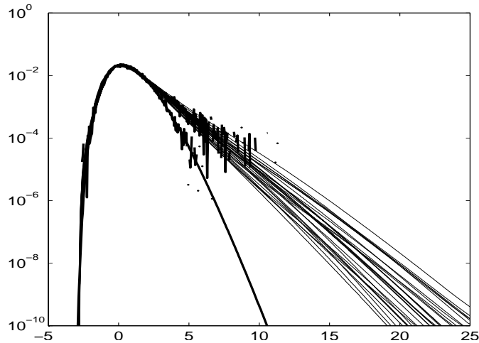
Fig. 6. Example 3: The thin solid lines (30 in number) are the crossing intensities \mu_N^s(u) using the proposed hybrid method, with sample size for simulated gamma processes \gamma_i is N = 100 ; the corresponding irregular solid line is MC estimate; The thicker solid line is the saddle point estimate \mu^s(u) with Gaussian forcing; the corresponding irregular solid line is the corresponding MC estimate.
