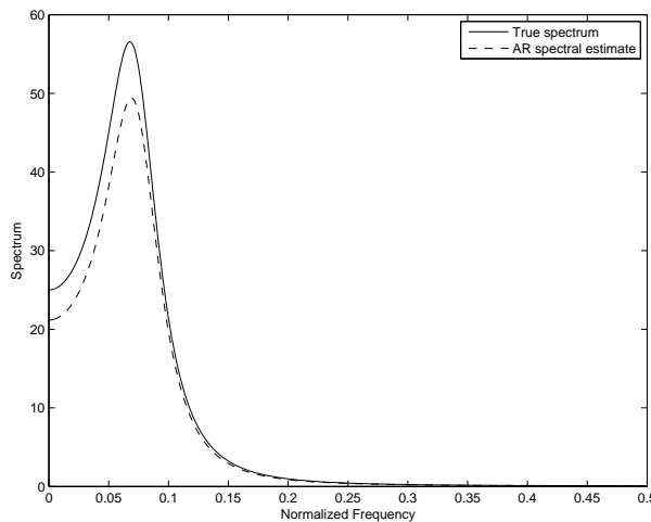
Figure 8: Parametric AR spectral estimation using the YW method. Both the estimated and the true spectrum is an AR(2) model.
