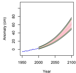
RCP 8.5
