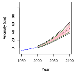
RCP 4.5
