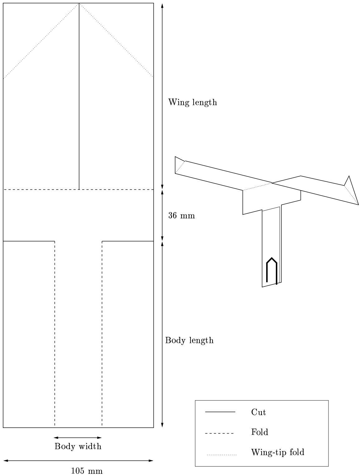
Figure 1: Design of CHC helicopters.
