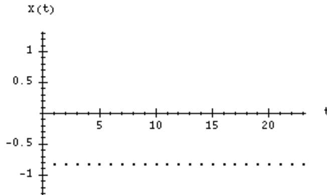
Figure 6.2. The process in Example 6.2 with \xi \sim N(0, 1) distributed.
