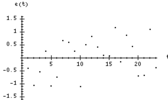
Figure 6.1. Discrete Gaussian white noise with variance \sigma^2 = 1 .
