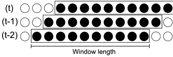
Fig. 6. Sliding-window model.
