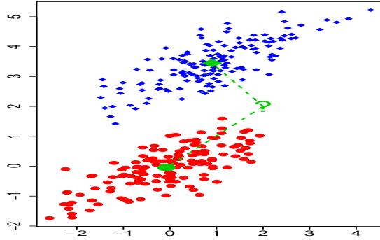
Figure 2.1: Illustration of distance-based classification. The centroid of each subsample in the training data is first computed by taking the sample mean or median. Then, for a future observation, indicated by query, it is classified according to its distances to the centroids.
