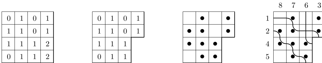
FIGURE 1. Permutation tableaux (1-hinge) of \pi = 36187425 . To the right is illustrated \pi(1) = 3 , \pi(2) = 6 and \pi(6) = 4
