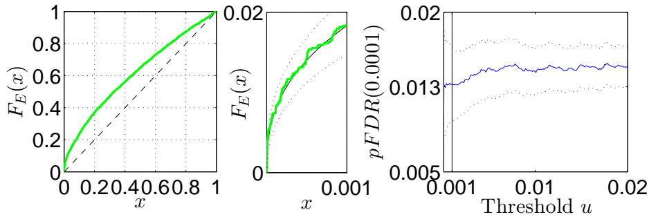
412 Fig. 1. Goodness of fit and parameter stability plots 413 for the KW analysis of the JIC4W data set
