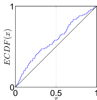
Fig. 3. Empirical cumulative distribution function of the Kolmogorov-Smirnov p-values from 93 fMRI brain scan data sets.
