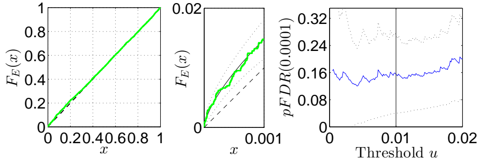
440 441 442 443 444 445 446 447 448 449 450 451 Fig. 2. Goodness of fit and parameter stability plots for the Q+K analysis of the JIC4W data set
