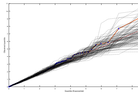
Fig. 5 Illustration of effect of size-biased sampling, left plot: Empirical quantiles for IDL supercentenarians who died 1980-1999 in USA plotted against quantiles of exponential distribution with estimated mean (red line, with observations in blue). To illustrate the statistical variation of such plots, we have simulated 100 data sets with the estimated mean for the US 1980-1999 data, and with the same 110 year birthdates and truncations, and inserted the empirical quantile lines (dotted) for these data sets in the plot .
