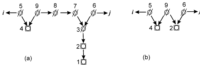
FIG. 4. (a) Example of a d-connecting ij -path in G_{\text{par}}^V relative to C with inner nodes 5, 4, 9, 8, 7, 3, 6 and (b) the corresponding active alternating ij -path in G_{\text{anc}}^{V,g} with inner nodes 5, 4, 9, 2, 6.
