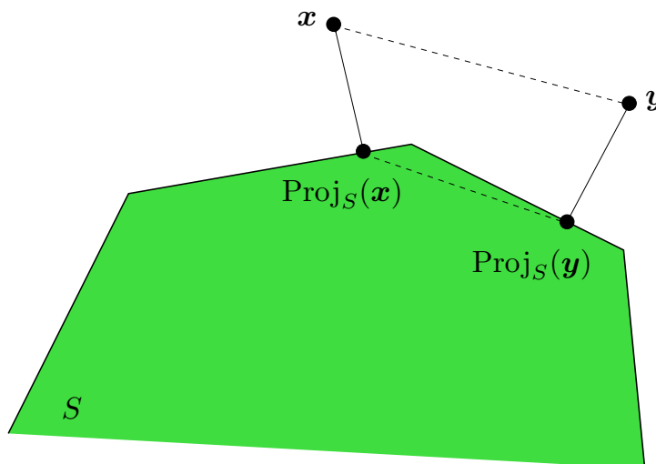
Figure 3: The projection operation is non-expansive.
