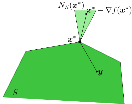
Figure 2: Normal cone characterization of a stationary point.
