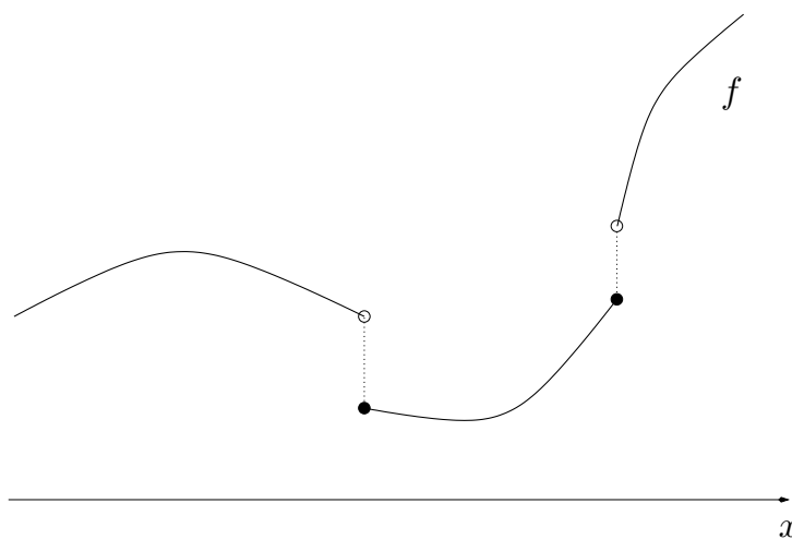
Figure 1: A lower semi-continuous function in one variable
