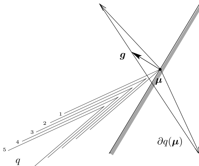
Figure 4: The half-space defined by the subgradient \mathbf{g} of q at \boldsymbol{\mu} . Note that the subgradient is not an ascent direction
