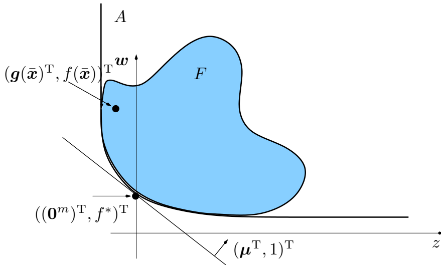
Figure 1: F := \{ (g(x)^T, f(x))^T \mid x \in X \} . A is convex; ((\mathbf{0}^m)^T, f^*)^T is not interior in A . A hyperplane through ((\mathbf{0}^m)^T, f^*)^T and supporting A is used to construct a Lagrange multiplier.
