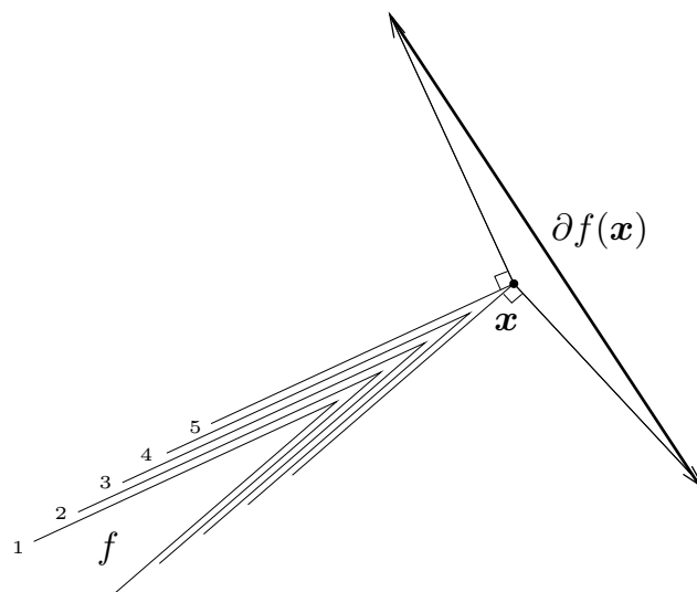
Figure 3: The subdifferential of a convex function f at x
