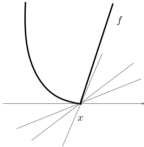
Figure 2: Three possible slopes of the convex function f at x
