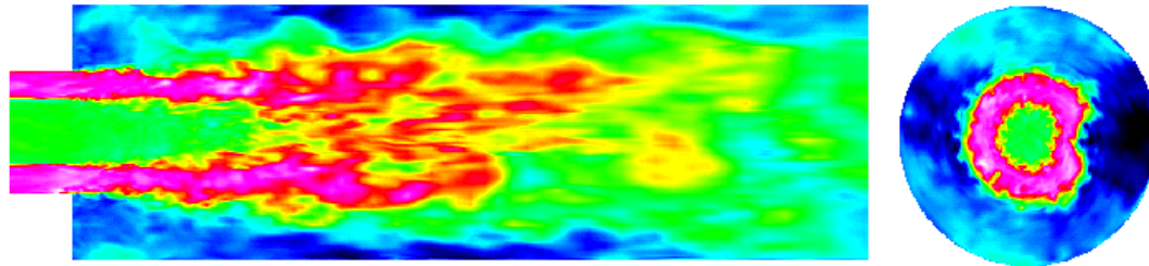
Swirling Coaxial Jet ( Sw=0.47 ) Axial Velocity
