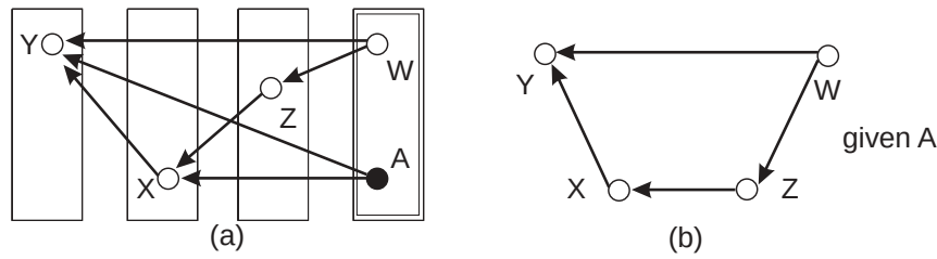
Figure 7. (a) Detailed representation of dependencies between variables listed and grouped in Figure 6. (b) Representation conditional on A , i.e. for two given levels of formal schooling.
